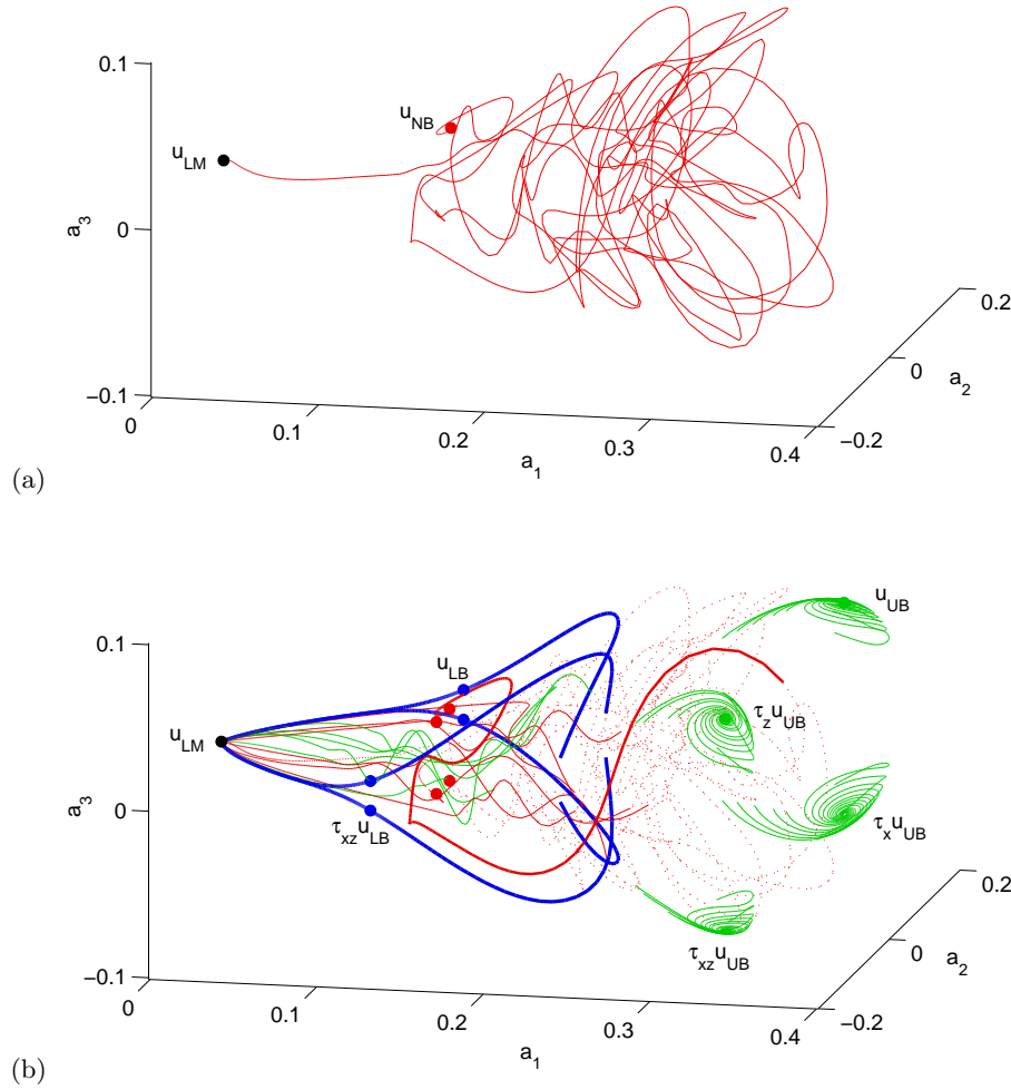
FIGURE 9. A transiently turbulent trajectory in the \mathbf{u}_{NB} unstable manifold, (a) in isolation (b) in relation to \mathbf{u}_{LB} , \mathbf{u}_{NB} , \mathbf{u}_{UB} , their half-cell translations, and their unstable manifolds (see figure 5 and figure 6 for more detailed labeling of these features). The final decay to laminar of several other trajectories in the unstable manifolds of \mathbf{u}_{NB} and \mathbf{u}_{UB} are also shown. The projection is the same as that of figure 6.
