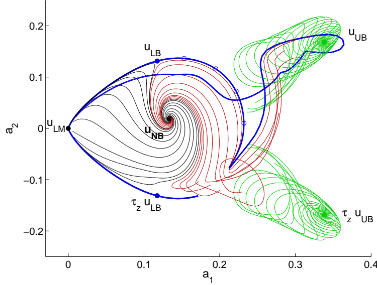
FIGURE 5. A state space portrait of plane Couette flow for Re = 400 and [L_x, L_y, L_z] = [2\pi/1.14, 2, 4\pi/5] , projected from 61 506 dimensions to 2. The labeled points are equilibrium (steady-state) solutions of the Navier-Stokes equation (see §3); the curved trajectories are fully-resolved time-dependent numerical integrations of Navier-Stokes projected onto the \mathbf{e}_1, \mathbf{e}_2 plane defined by (4.3), with the projection a_n = (\mathbf{u}, \mathbf{e}_n) defined by (4.1). The laminar equilibrium is \mathbf{u}_{LM} ; the equilibria labeled \mathbf{u}_{LB} , \mathbf{u}_{NB} , and \mathbf{u}_{UB} are shown in figure 3. W_{LB}^u , the 1d unstable manifold of the ‘lower-branch’ equilibrium \mathbf{u}_{LB} , and \tau_z W_{LB}^u , its half-cell translation in z , are shown with thick blue lines. W_{NB}^{u(1,2)} , a 2d portion of the unstable manifold of \mathbf{u}_{NB} , is shown with thin black and red spirals emanating from \mathbf{u}_{NB} . Similarly, the thin green lines spirally out of \mathbf{u}_{UB} and \tau_z \mathbf{u}_{UB} indicate W_{UB}^{u,S} and \tau_z W_{UB}^{u,S} , the 2d unstable manifolds of \mathbf{u}_{UB} and its half-cell translation \tau_z \mathbf{u}_{UB} . Open dots along W_{LB}^u show initial conditions for Newton-GMRES searches used to find \mathbf{u}_{NB} . The plane of the projection is defined in terms of the equilibrium solutions; it is dynamically invariant and independent of the numerical representation. See §4.2, §4.3, and §3.2 for discussions of the projection, dynamics, and numerical discretization.
